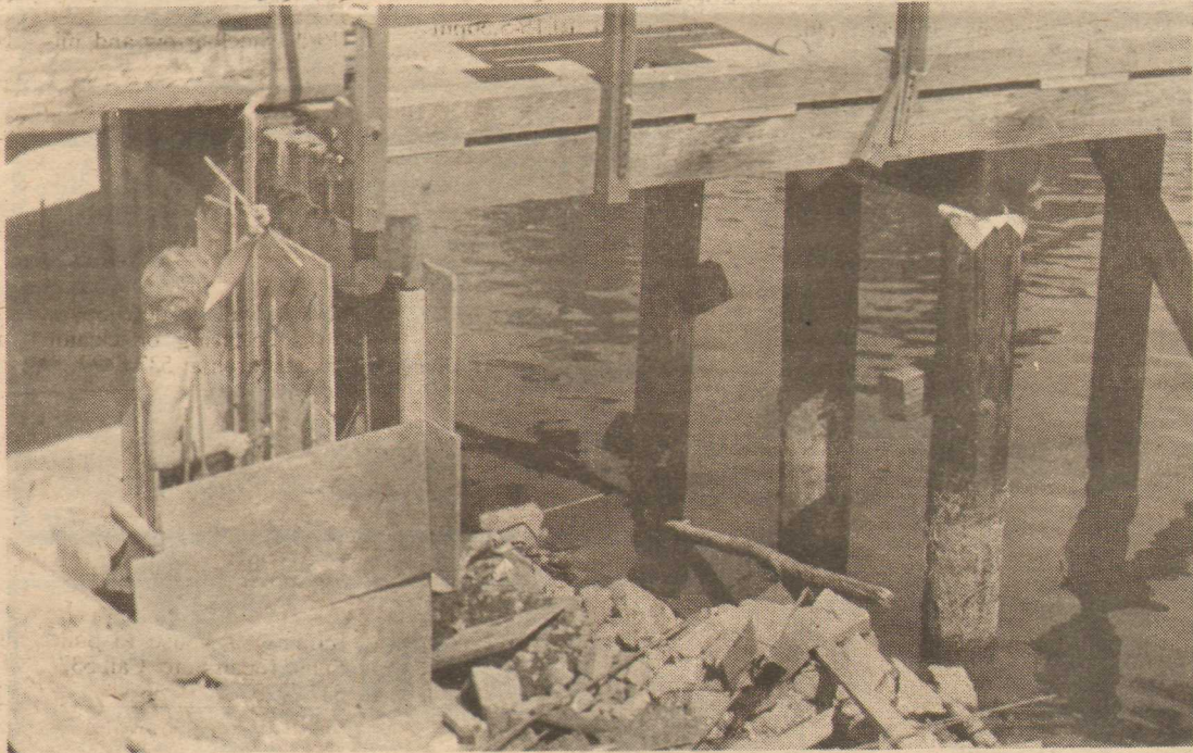
WORKMAN constructs the wall forms preparatory to the pouring of the cement base to wharf approach.
