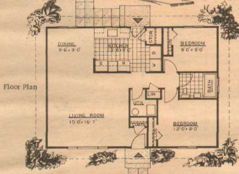
Size 34' x 24' 2 Bedroom Home
